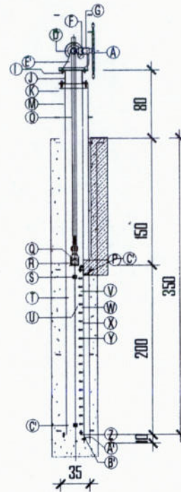
TAMPAK SAMPING
